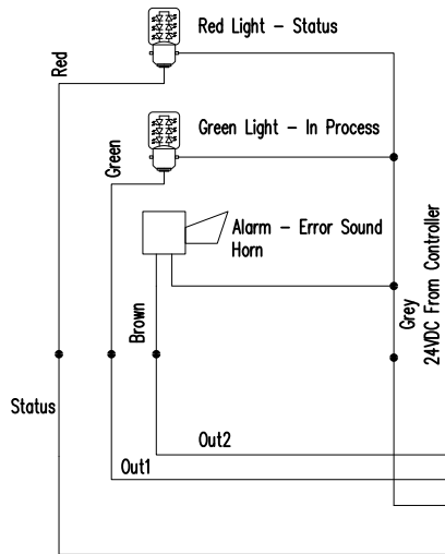
Optional connection for Warning Signals of 24VDC LED Lights and Horn
