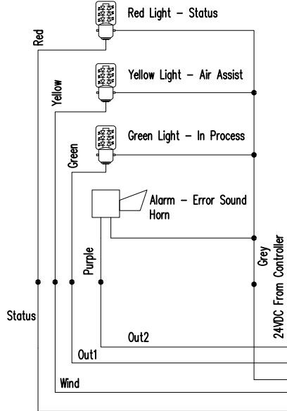
Optional connection for Warning Signals of 24VDC LED Lights and Horn
